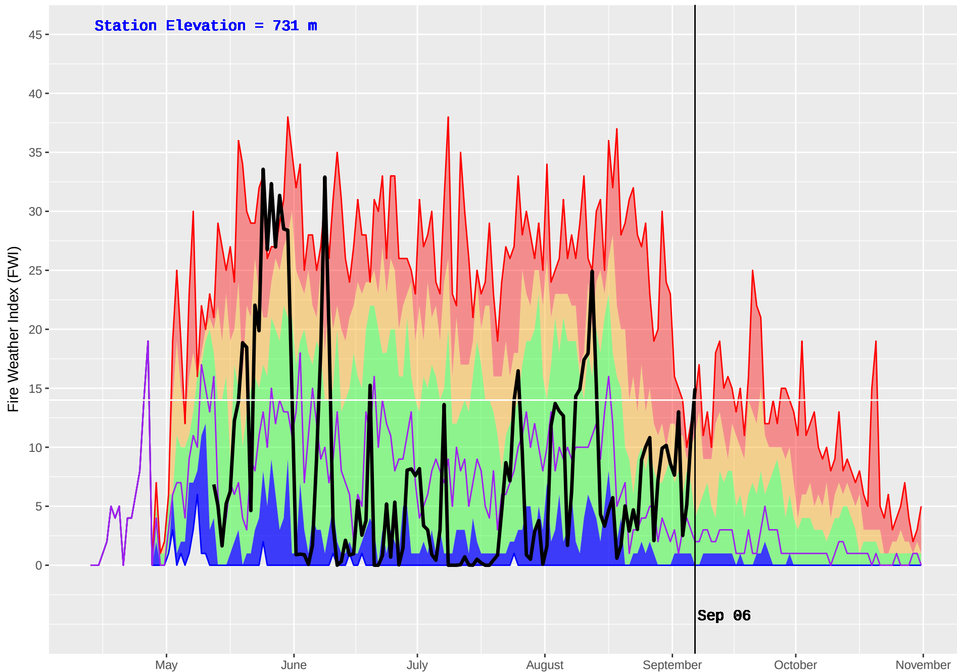
FIRESIDE (440) : Historical (1996–2016) and Current (2017) Noon Fire Weather Index (FWI)
