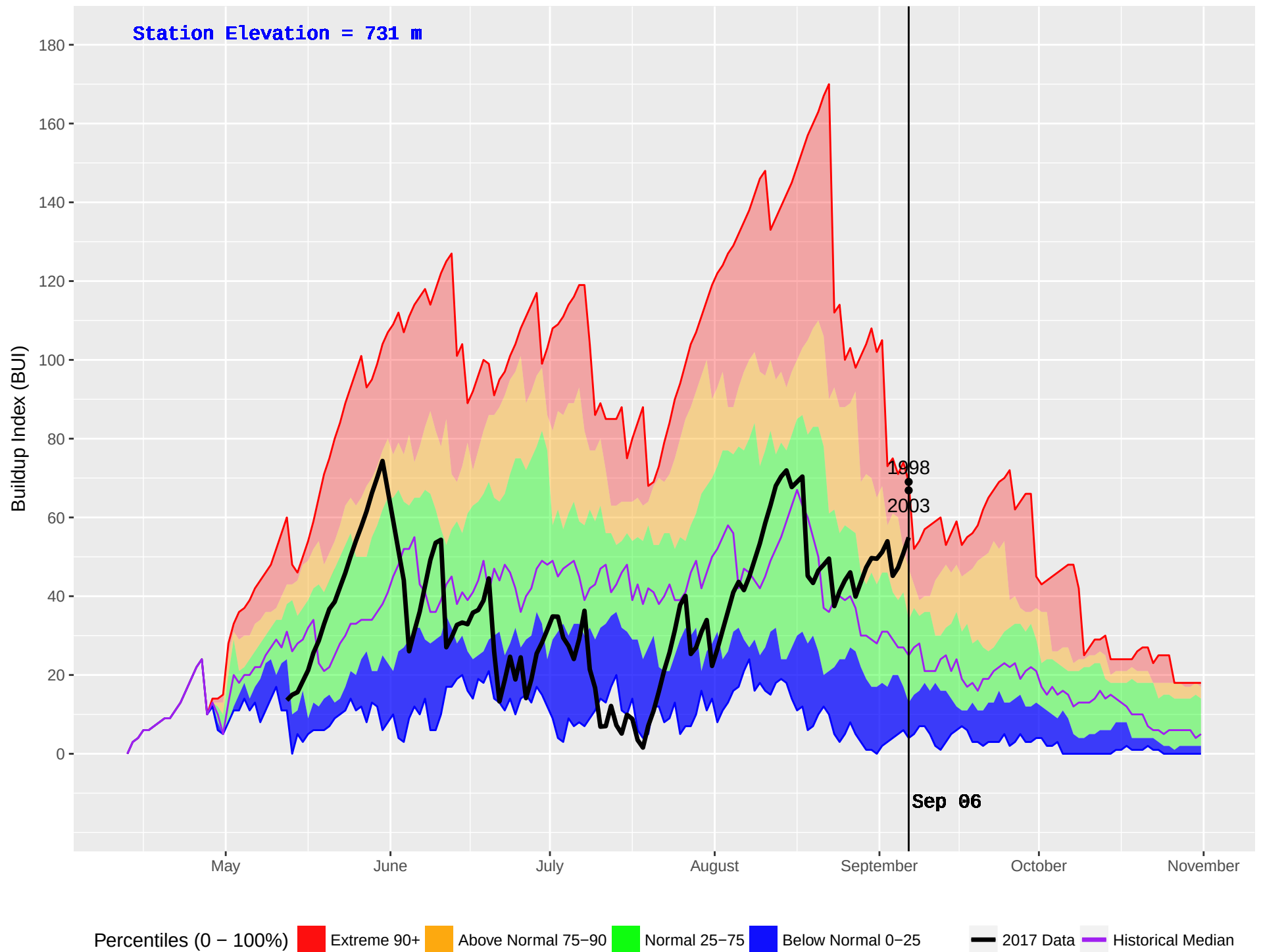
FIRESIDE (440) : Historical (1996–2016) and Current (2017) Noon Buildup Index (BUI)
